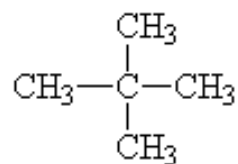
2,2-dimethylpropane
